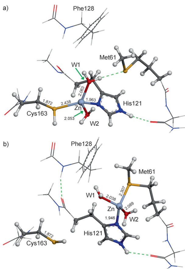
Figure 5. Optimized structures of probable zinc binding sites in caspase-3: a) the catalytic dyad (ZnCH) and b) His121 and Met61 (ZnMH). Zinc–ligand bond lengths (Å) are shown. W1 and W2 are water molecules.
